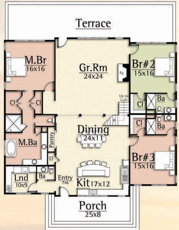
Main Level 2,800 square feet
