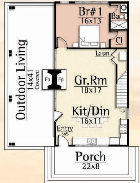
Main Level 943 square feet
